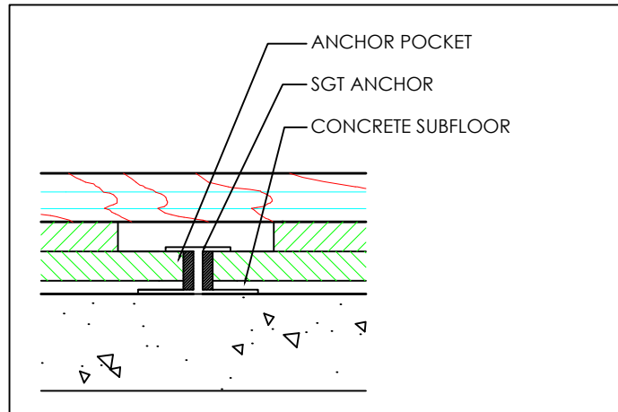
OPTIONAL SGT ANCHOR SYSTEM PROVIDING MIN 900LB TENSION
